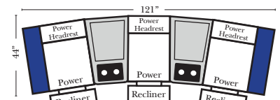
Recl 3C Sofa w/2 Large Wedge Console Arms-53849
